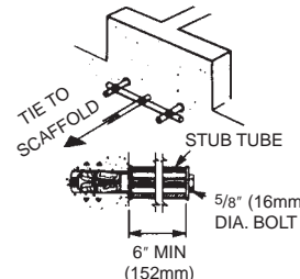
SECURED TO EMBEDDED TIES IN CONCRETE
