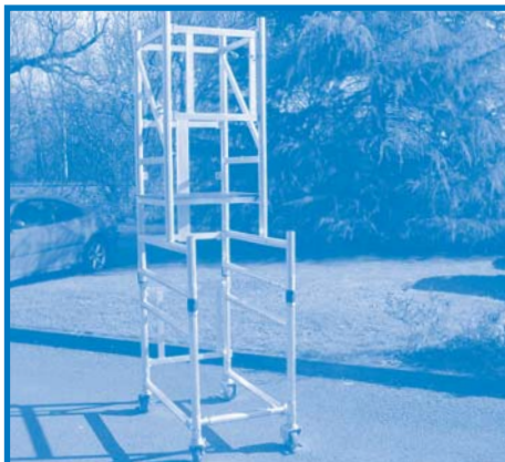
8. Using two people lift the assembled folding frame on top of the booster unit locating the uprights of the folding unit into the cups on top of the booster unit. Ensure all of the spring loaded pins in the cups are engaged into the holes in the frame.
