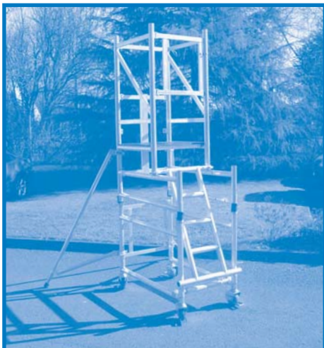
10. Fit stabilisers to front uprights of unit ensuring wing nuts are tightened
