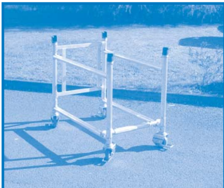
7. Remove the feet or castors from the bottom of the folding frame (see 1. on previous page) and re fit them into the bottom of the booster frame retaining them in the same manner. Stand the frame on its feet or castors and open it out to form a rectangle. Clip the short brace into position over the pegs provided.
